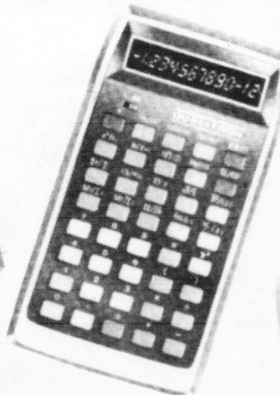
Model 1421 Advanced Programmable Scientific
