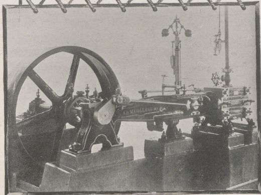
Engine Built by the Students of State College.
