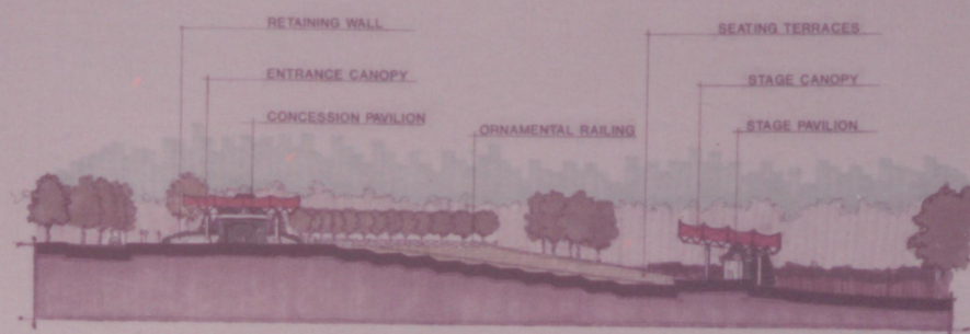
SECTION A-A 1" = 30'
