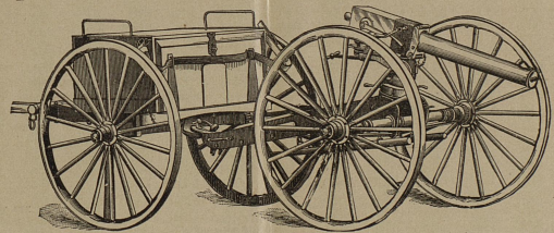
Gardner Gun-carriage and Limber.
